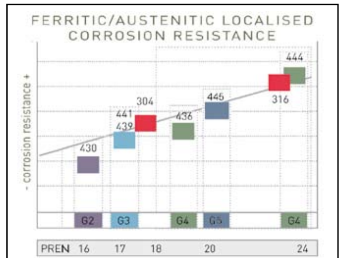
The PREN (Pitting Resistance Equivalent Number), \%Cr+3.3\%Mo+0.16\%N , is a measure of the pitting-corrosion resistance of a stainless steel grade in a chloride-containing environment. The higher the PREN the greater the corrosion resistance.
